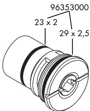
Ecostat iBox 95036000
