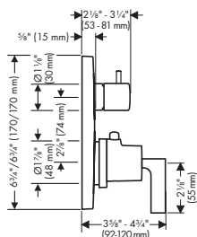
AXOR Soft Cube 04985XX0
