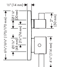
AXOR Soft Cube 04985XX0
