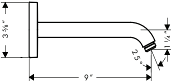
AXOR 230 Showerarm Square / SoftSquare 26430XX1 / 26968XX1
