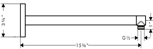
AXOR 390 Showerarm Square / SoftSquare 26436XX1 / 26967XX1
