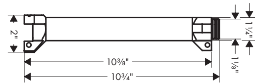
AXOR Rough for Large Shelf / Extension Pipe 40878180
