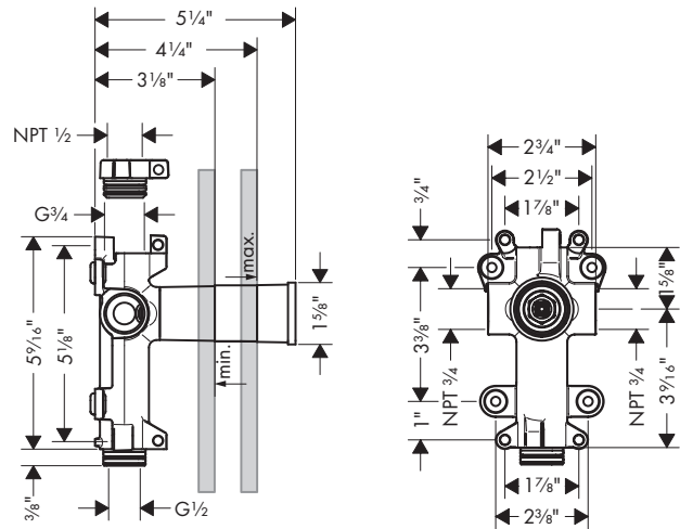
AXOR Shower Module 28486181
