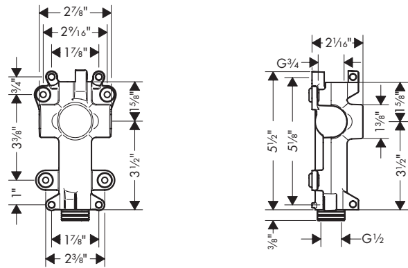
AXOR Rough for Small Shelf / Extension Pipe 40877180
