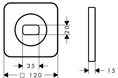
AXOR ShowerSphere 120/120 softsquare 39769XX0
