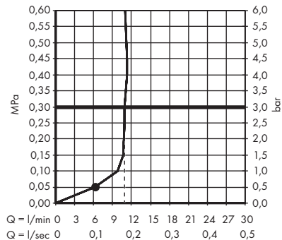
AXOR Archivio 240 1jet EcoSmart 34054XX0
