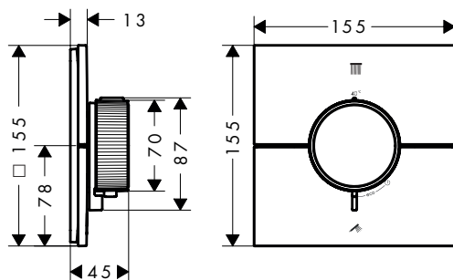
AXOR ShowerSelect ID square 36752XX7
