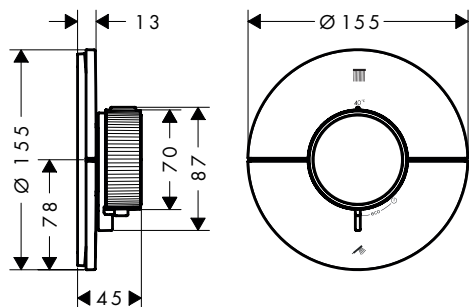
AXOR ShowerSelect ID round 36750XX7
