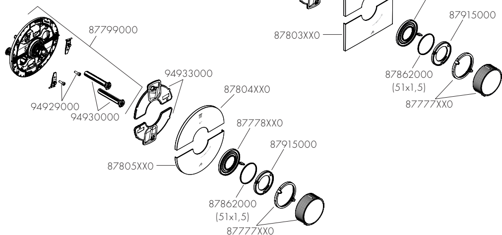
AXOR ShowerSelect ID round 36750XX7
