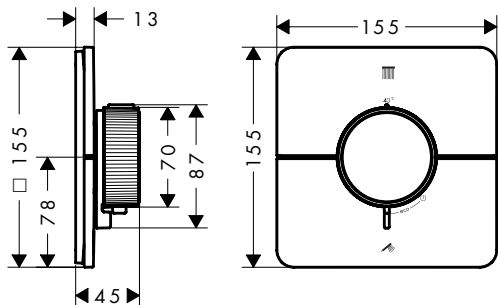
AXOR ShowerSelect ID softsquare 36754XX7
