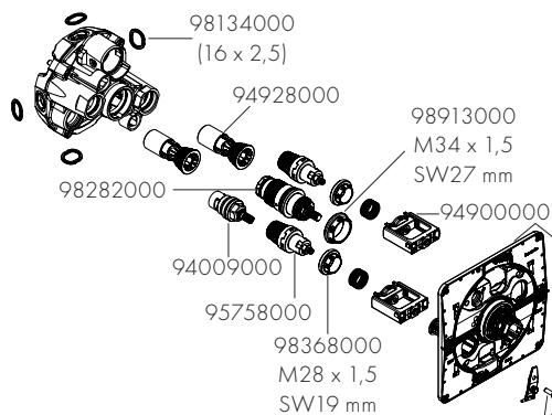
AXOR ShowerSelect ID round 36750XX7
