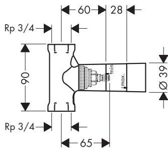
AXOR DN20 (3/4") 16970180
