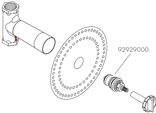
AXOR DN20 (3/4") 16970180
