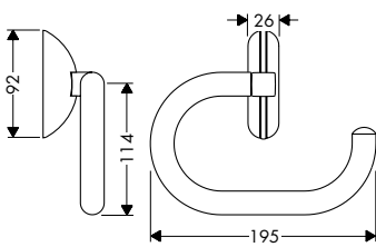
Arco 40621XXX
