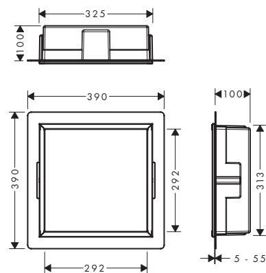
XtraStoris Original 300 x 300 x 100 mm
