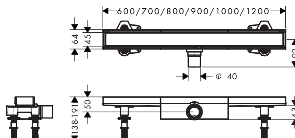
RainDrain Compact flat installation tile
