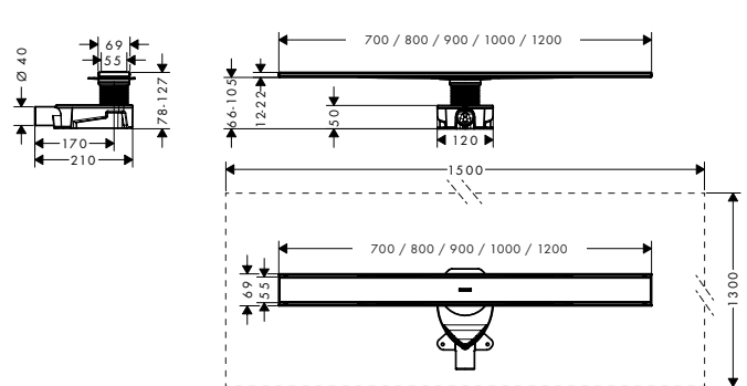
RainDrain Allround flat installation
