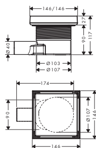
RainDrain Brilliance 150 x 150
