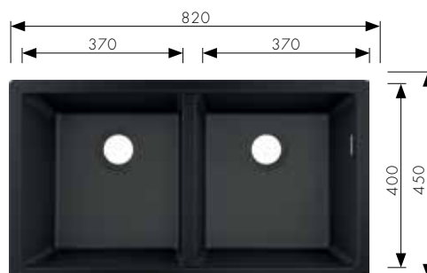
Undermount sink 370/370
