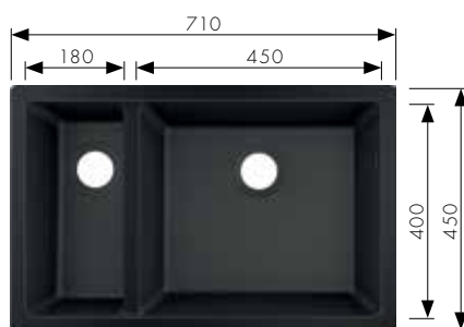
Undermount sink 180/450
