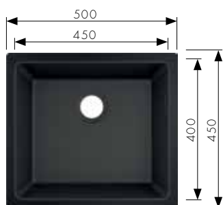
Undermount sink 450
