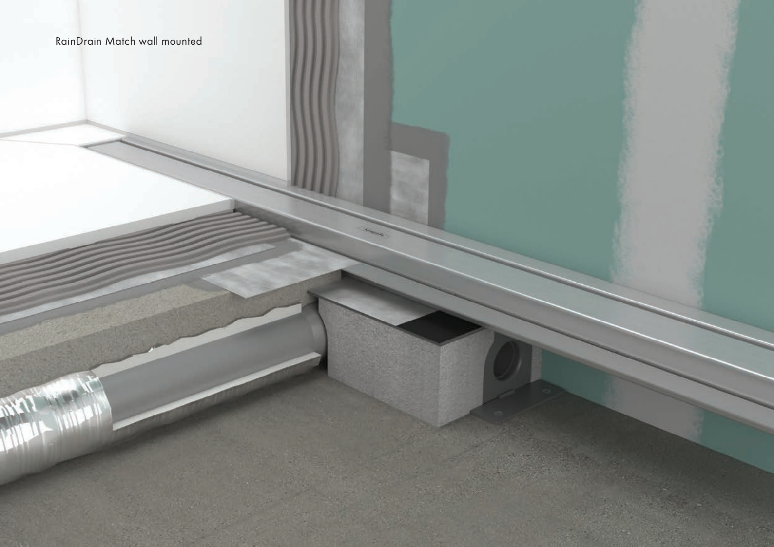
RainDrain Flex wall mounted
