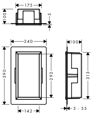
XtraStoris Original 300 x 150 x 100 mm
