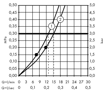
Flow diagram Rainmaker Select 460 3jet Showerpipe # 27106, -400
