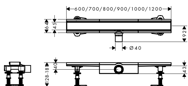
RainDrain Compact flache Installation
