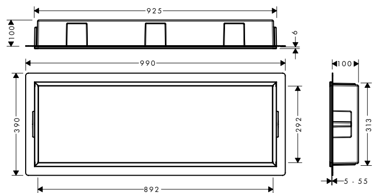
XtraStoris Original 300 x 900 x 100 mm
