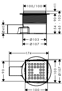
RainDrain Point 100 x 100
