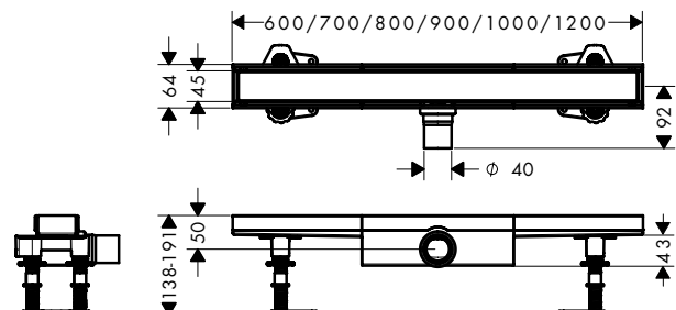
RainDrain Compact flache Installation Fliese
