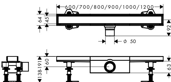
RainDrain Compact Standardinstallation Fliese
