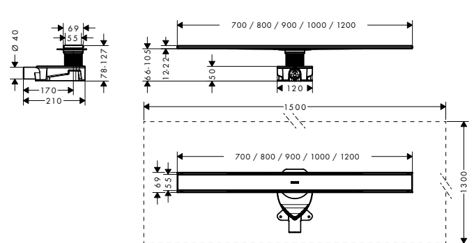
RainDrain Allround flache Installation
