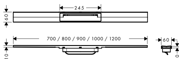
RainDrain Flex frit i gulv
