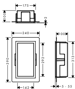
XtraStoris Individual 300 x 150 x 100 mm
