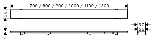
RainDrain Rock
