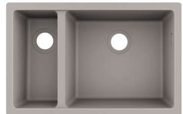
Under-mount sink 180 x 450 Graphite black: #43433170 Stone grey: #43433290 Concrete grey: #43433380
