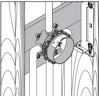
Mounting between two wall studs
