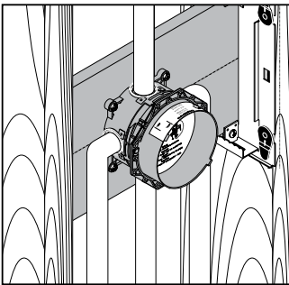
Mounting between two wall studs
