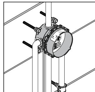
Installation in front of the wall (shown with variable spacers)
