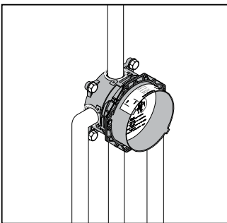
Installation on the wall
