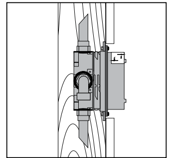
Installation with #96615000 installation set
