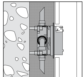
Installation in front of the wall (shown with variable spacers)
