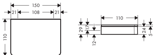
AXOR Universal Accessories 42840XX0 / 42840XX7
