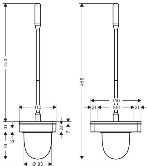
AXOR Universal Accessories 42835XX0 / 42835XX7
