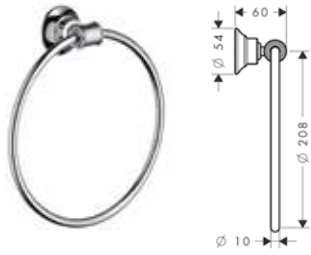
Handtuchring , aus Metall, Wandmontage Anneau porte-serviette, en métal, montage mural Porta asciugamani ad anello, in metallo, montaggio a parete
